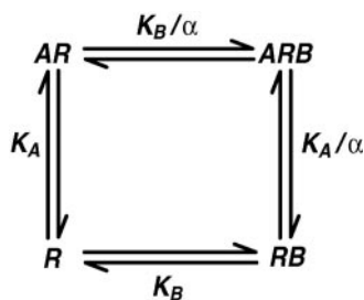
Fig. 1. The allosteric TCM, where R denotes the receptor; A and B denote the orthosteric and allosteric ligands, respectively; K_A and K_B denote their respective equilibrium dissociation constants; and \alpha denotes a cooperativity factor that governs the magnitude and direction of the allosteric interaction between the two ligands when they both occupy the receptor. Values of \alpha greater than 1 denote positive binding cooperativity (enhanced affinity), values less than 1 denote negative binding cooperativity, and values equal to 1 denote neutral binding cooperativity.
