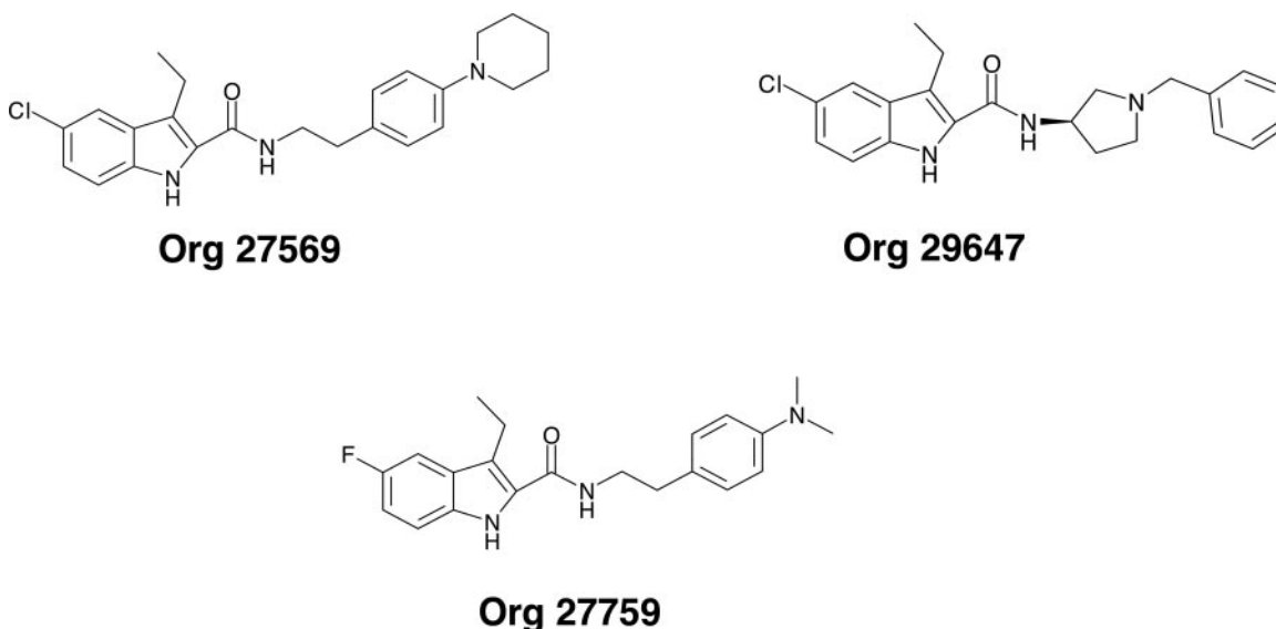
Fig. 2. Structure of Organon compounds Org 27569-0, 5 Org 27759-0, and Org 29647-1.
